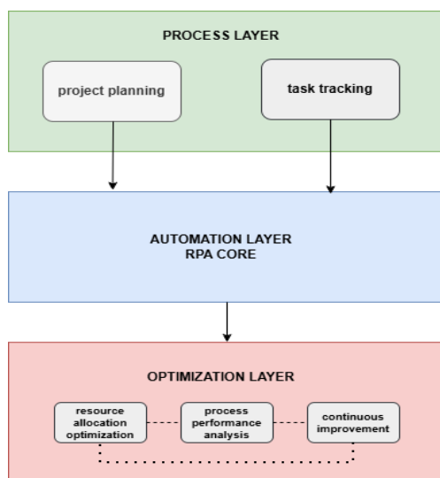
Figure 2. Structure of the three-layer framework for optimizing IT Project Management with RPA and AI agents. Source: authors' own result
